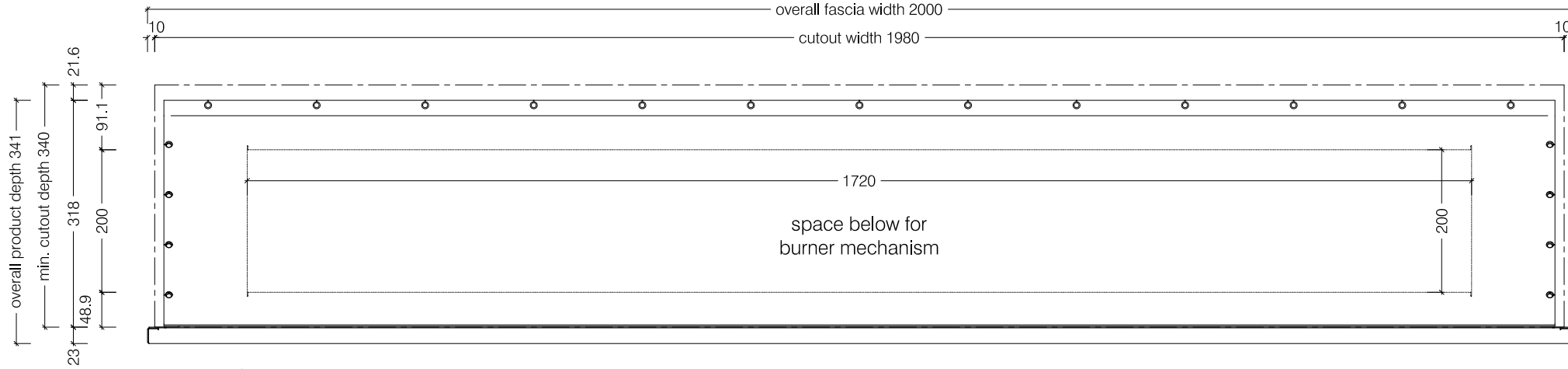
Top View
