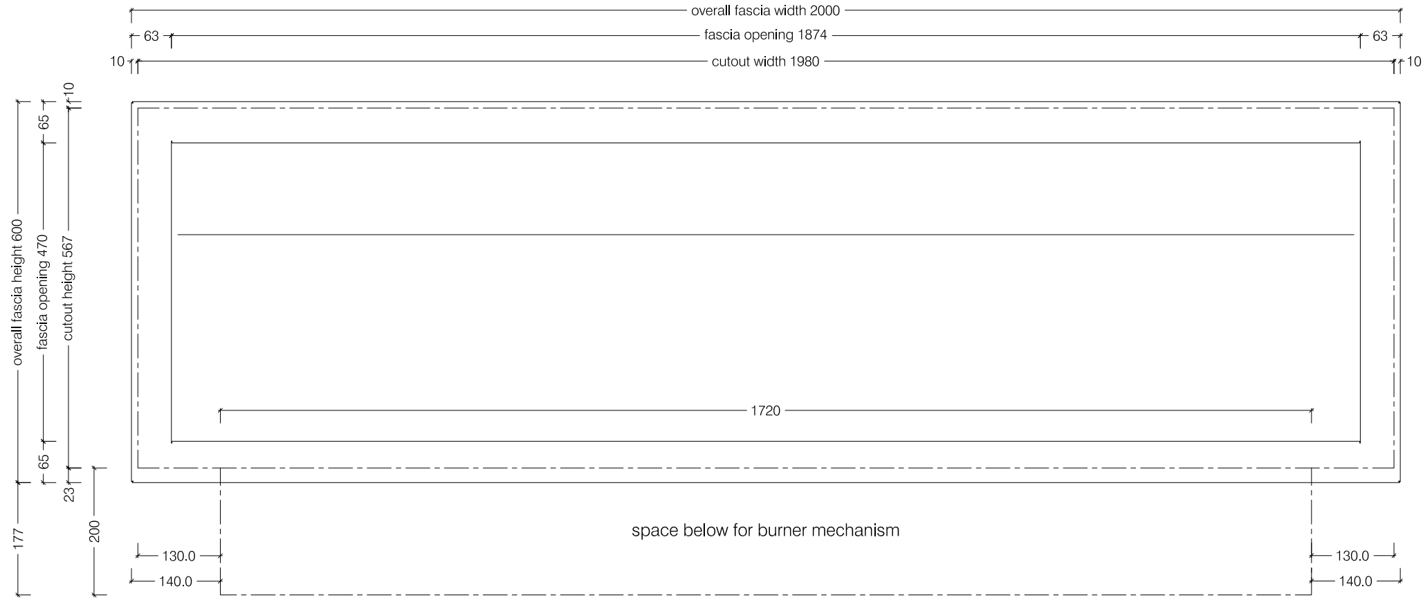
Front View
