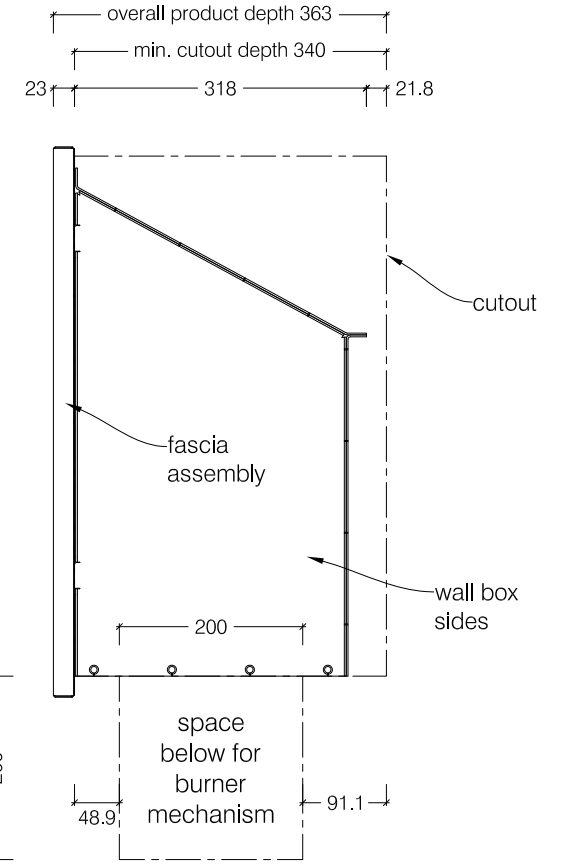
Side View
