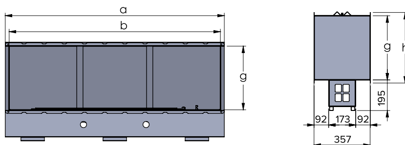
DIMENSIONS FOR SINGLE & DOUBLE SIDED UNITS WITH FRAME
