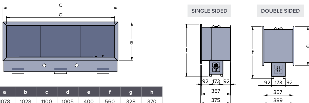
DIMENSIONS FOR SINGLE & DOUBLE SIDED UNITS WITH FRAME
